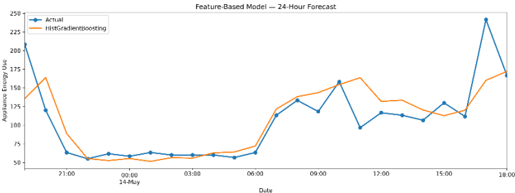
Figure 7: Comparison of observed and predicted hourly appliance energy consumption using the HistGradientBoosting feature-based forecasting model over the 24-hour prediction horizon
