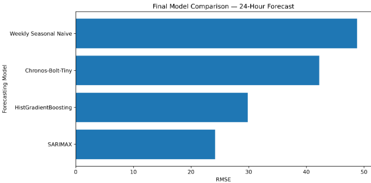
Figure 9: Comparison of forecasting accuracy (RMSE) for the evaluated forecasting models over the common 24-hour test period.
